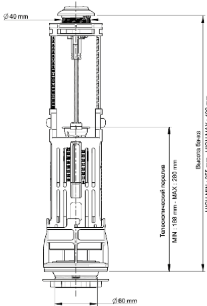
double push, telescopic overflow
