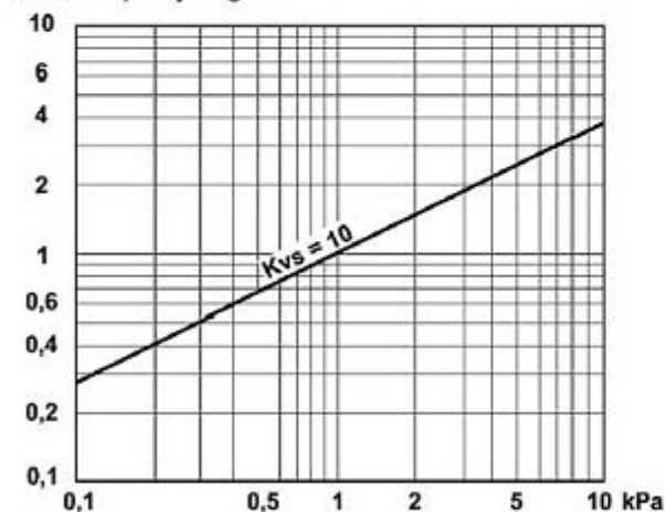
m^3/h Capacity diagram
