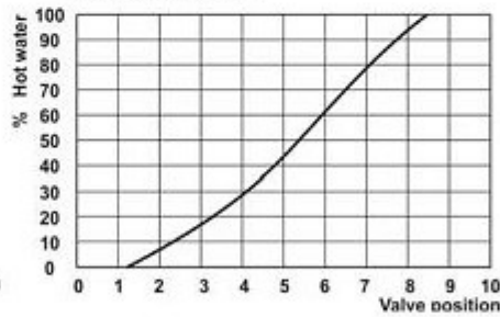
Mixing characteristic
