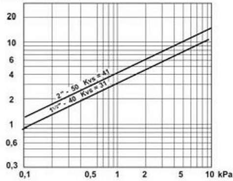
m 3 /h Capacity diagram
