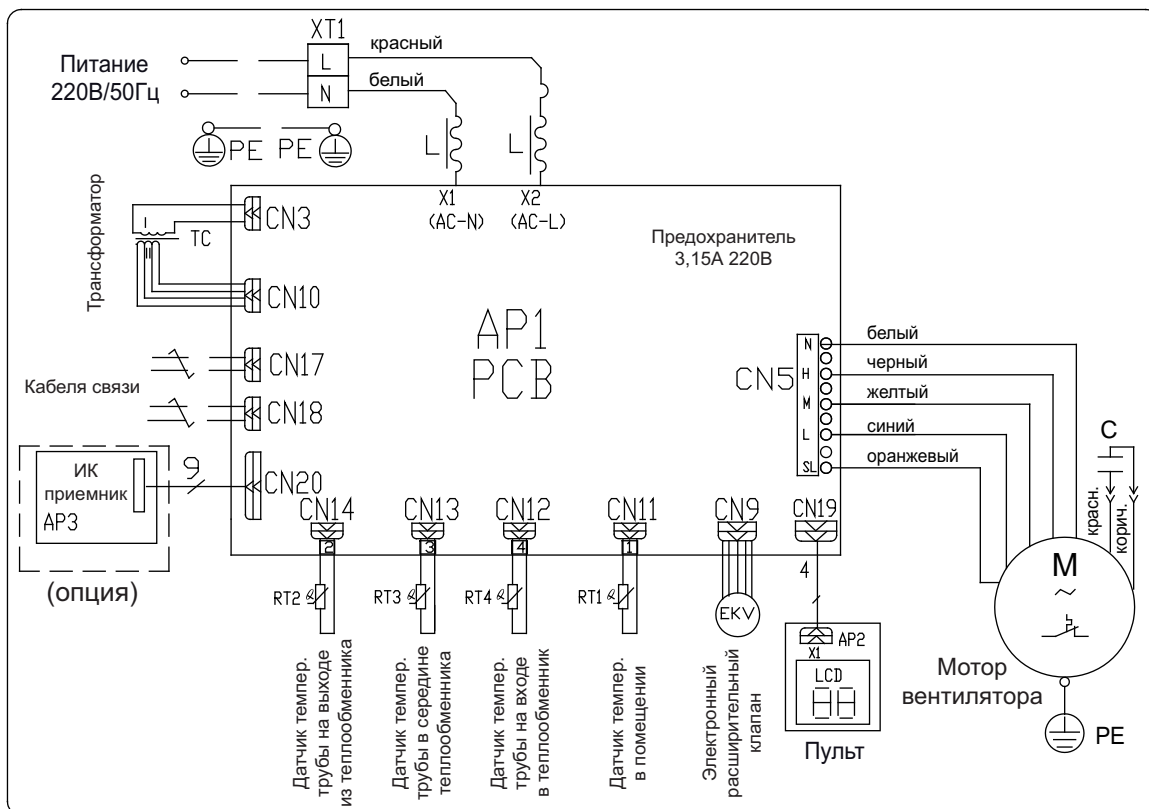
TMV-R90P/NaB-K, TMV-112P/NaB-K, TMV-140P/NaB-K
