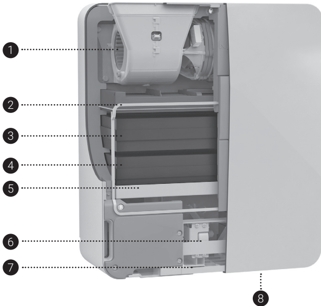
Figure 1. Device layout
