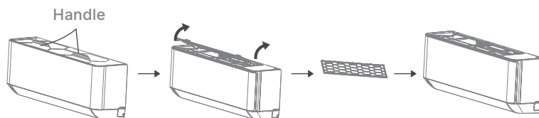
Figure 10 — Removing and installing the air filter frame
