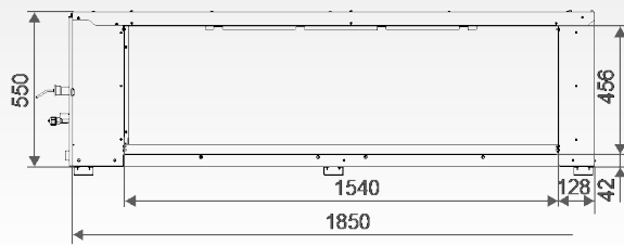
Dimensions of the air outlets:
