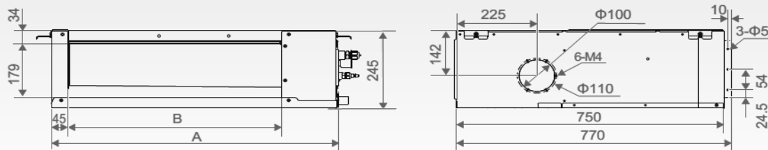
External dimension, air outlet size, and size of fresh air outlet:
