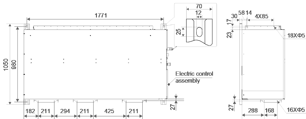
Dimensions of lugs and the screw hole of air outlet/inlet flange:
