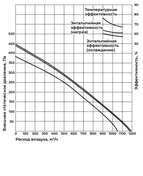
PVS-1100
