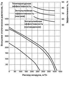
PVS-1100
