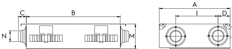
PVS 200-450
