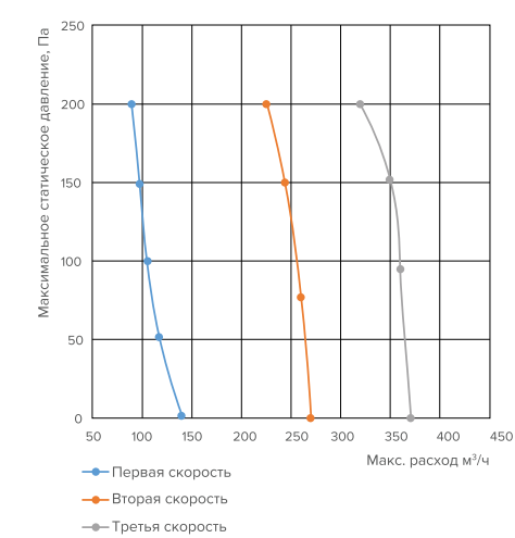
VR-350 inv
