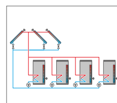
Solar system with 3 collector fields and 4 stores, valve/ pump logic
