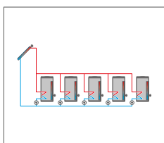
Solar system with 5 stores, pump logic
