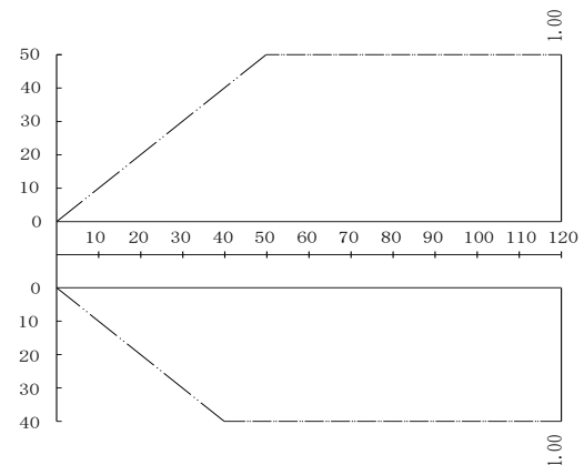
Figure 2-8.6: 160 model rate of change in heating capacity
