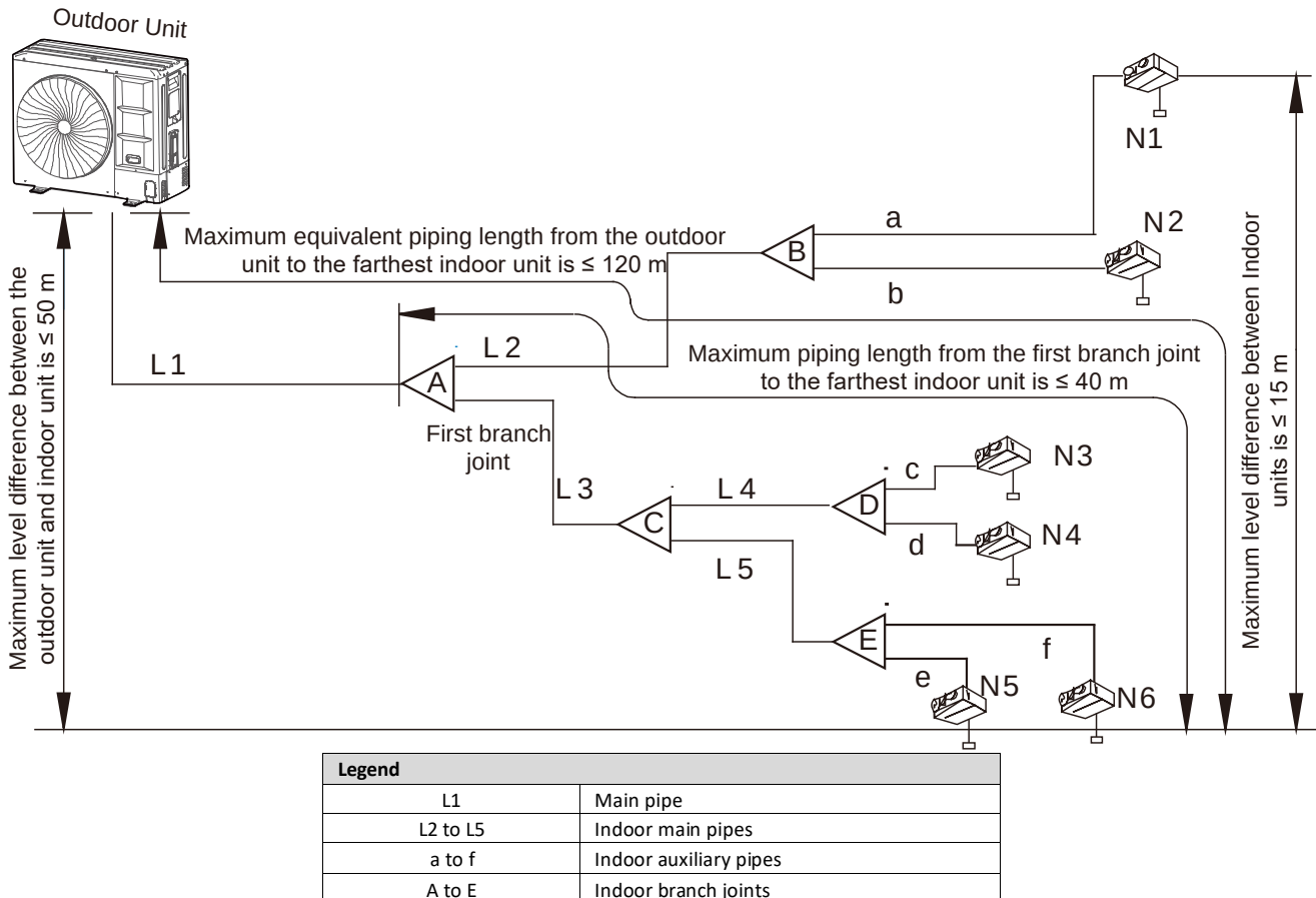
Figure 3-3.1: Permitted refrigerant piping lengths and level differences
