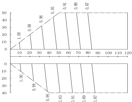
Figure 2-8.5: 160 model rate of change in cooling capacity
