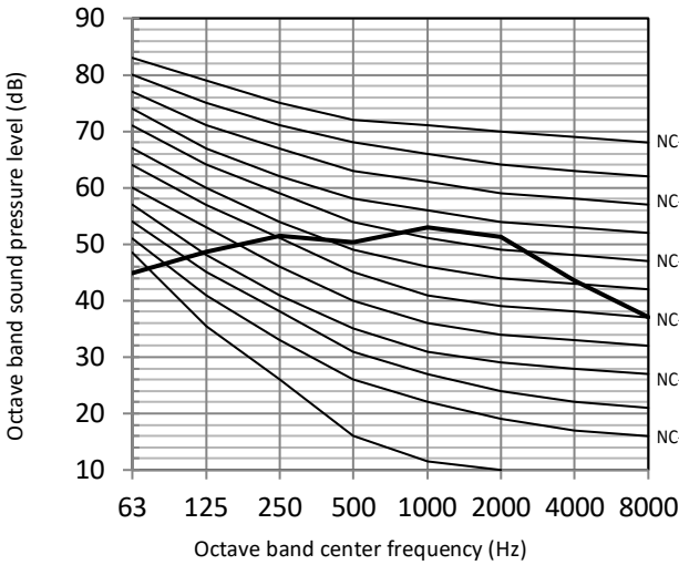
Figure 2-10.2: 120 model octave band level
