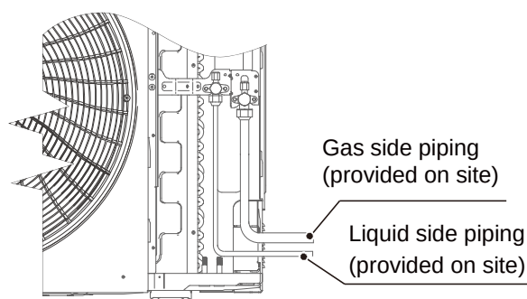
Figure 3-4.11: The connection method of the rightward outlet pipe
