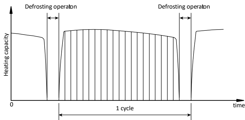
Figure 2-8.7: Defrosting cycle
