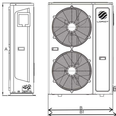
LAC-48/60A-OUT
