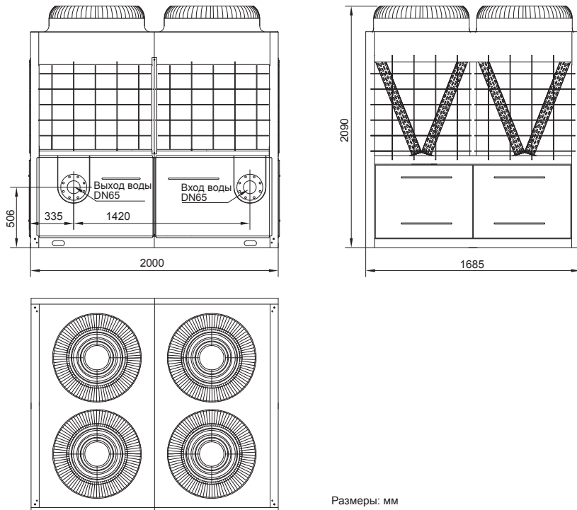
LUC-FHMA130CAW
