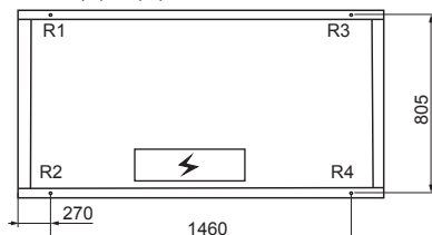
LUC-F(D)HD(M)A65CAW
