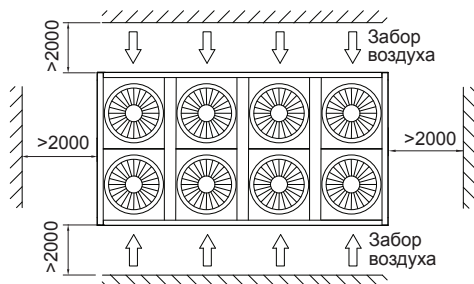
LUC-FHMA250CAW
