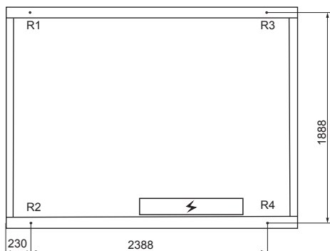
LUC-FHMA185CAW
