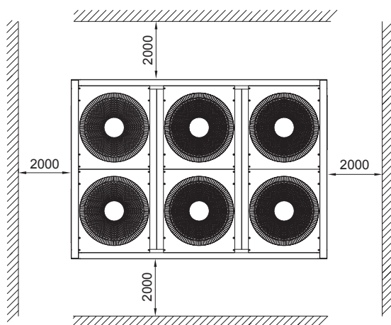
LUC-FHMA250CAW
