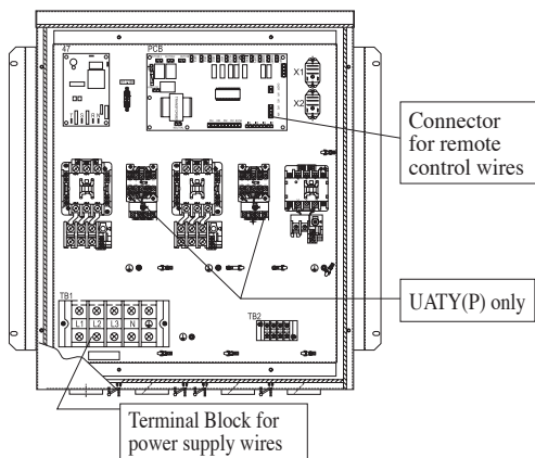
CONTROL MODULE UAT(Y)(P)300A
