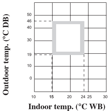
Cooling Only Unit & Cooling Mode For Heat Pump Model
