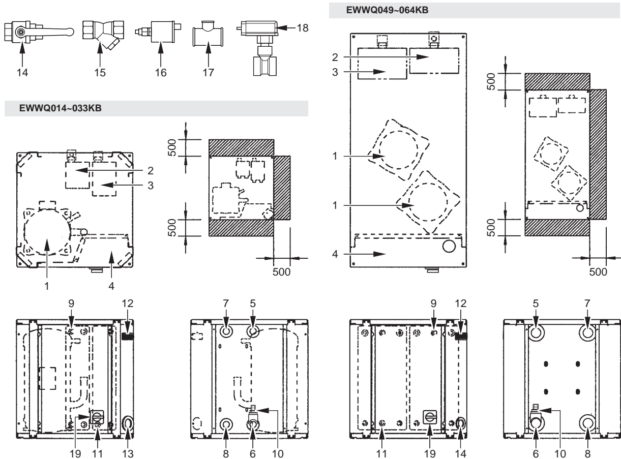
Figure – Principaux composants
