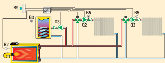
Diagram of a system on a hydraulic manifold
