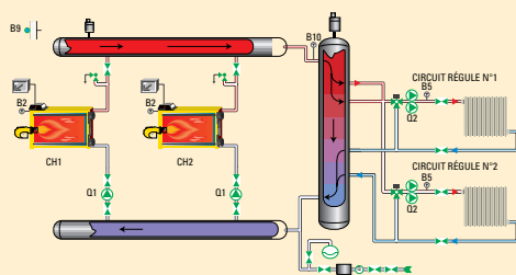
Diagram of a system on a hydraulic separation bottle
