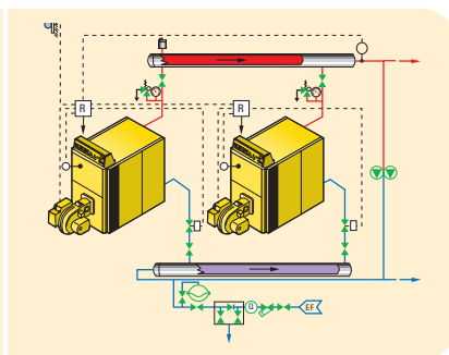
■ Diagram 3 1 common recycling pump for maximum 2 boilers
