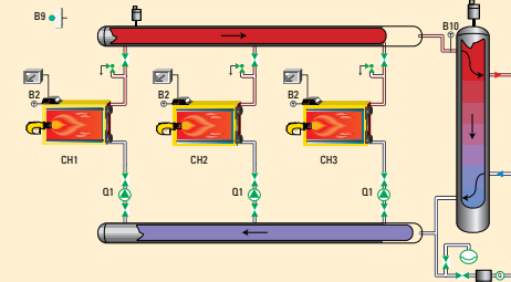
Diagram of a system on a hydraulic separation bottle
