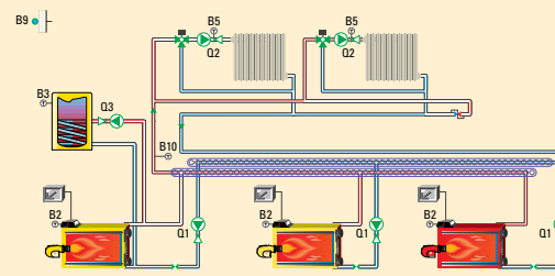
Diagram of a system on a hydraulic manifold
