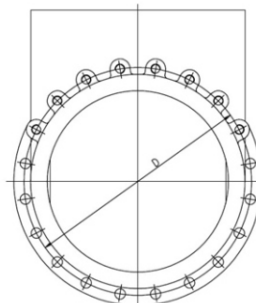
DN450-DN600
