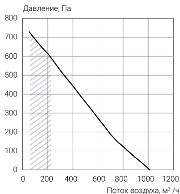
ECT PV-R 1250
