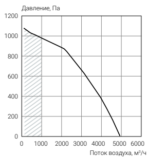
ECT PH-R 3700/4300
