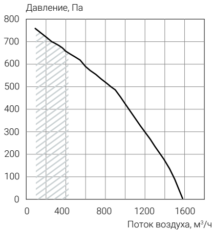
ECT PV-R 1500
