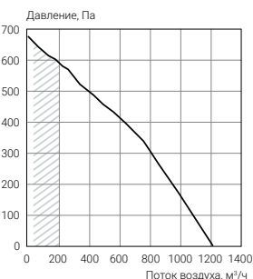
ECT PH-R 1000
