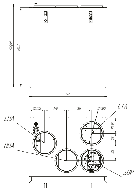
ECT PV-R 500
