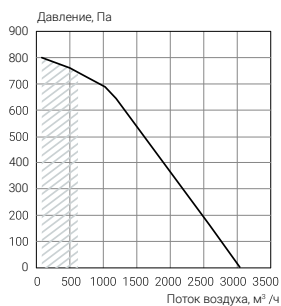
ECT PH-R 2950
