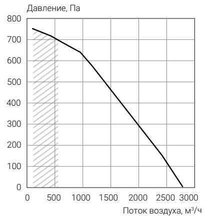
ECT PV-R 2950
