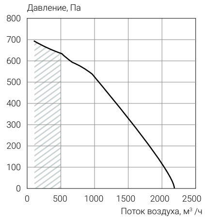
ECT PV-R 1850
