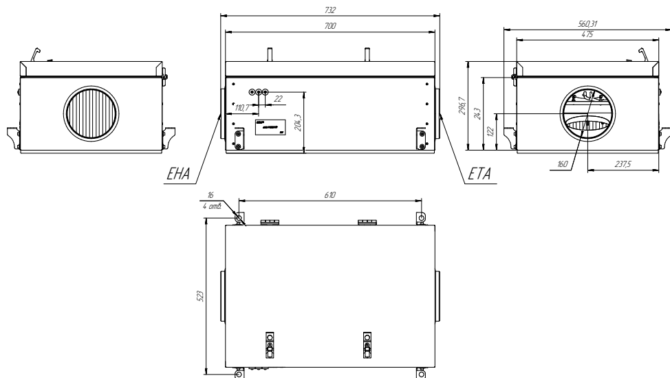
ECT PF-V 950-4
