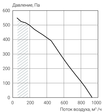
ECT PV-R 1000
