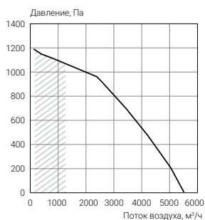
ECT PH-R 5000
