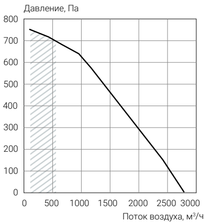
ECT PV-R 2350
