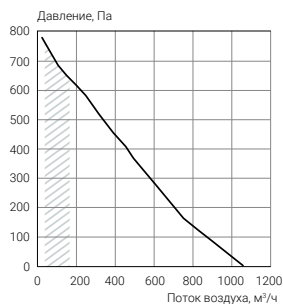
ECT PH-R 850
