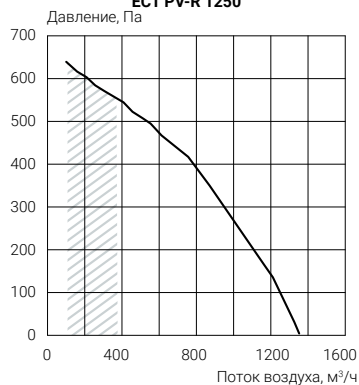
ECT PV-R 1250
