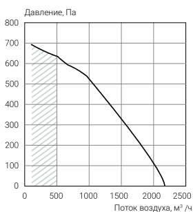
ECT PH-R 1850
