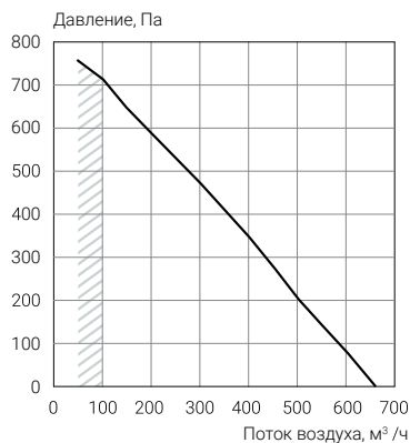
ECT PV-R 850
