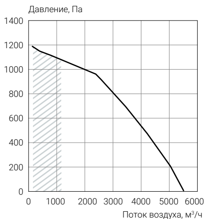
ECT PV-R 5000
