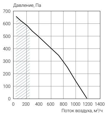
ECT PV-R 1000
