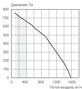
ECT PH-R 1500
