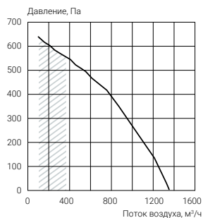
ECT PH-R 1250
