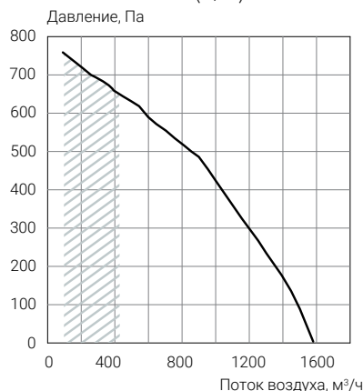
ECT PV-R 1500-E4.5-(L/R)-5 ECT PV-R 1500-W- (L/R)-4
