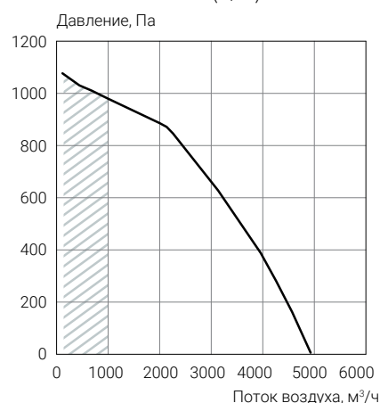
ECT PV-R 3700-E9.0-(L/R)-5 ECT PV-R 3700-W- (L/R)-5
