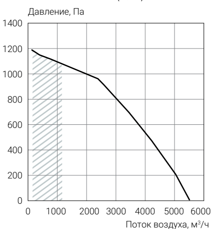
ECT PV-R 5000-E13.5-(L/R)-5 ECT PV-R 5000-W- (L/R)-5
