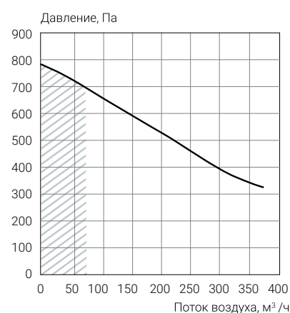
ECT PF-R 400-E1.0-R-4 Pro ECT PF-R 400-W-R-4 Pro
