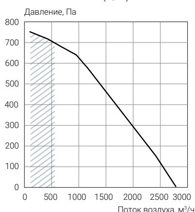
ECT PV-R 2350-E7.5-(L/R)-5 ECT PV-R 2350-W- (L/R)-4
