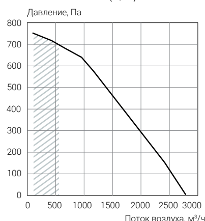
ECT PV-R 2950-E7.5-(L/R)-5 ECT PV-R 2950-W- (L/R)-4
