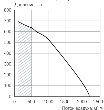
ECT PV-R 1850-E4.5-(L/R)-5 ECT PV-R 1850-W- (L/R)-4
