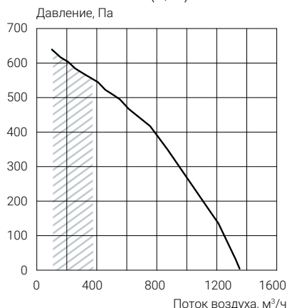
ECT PV-R 1250-E4.5-(L/R)-5 ECT PV-R 1250-W-(L/R)-4
