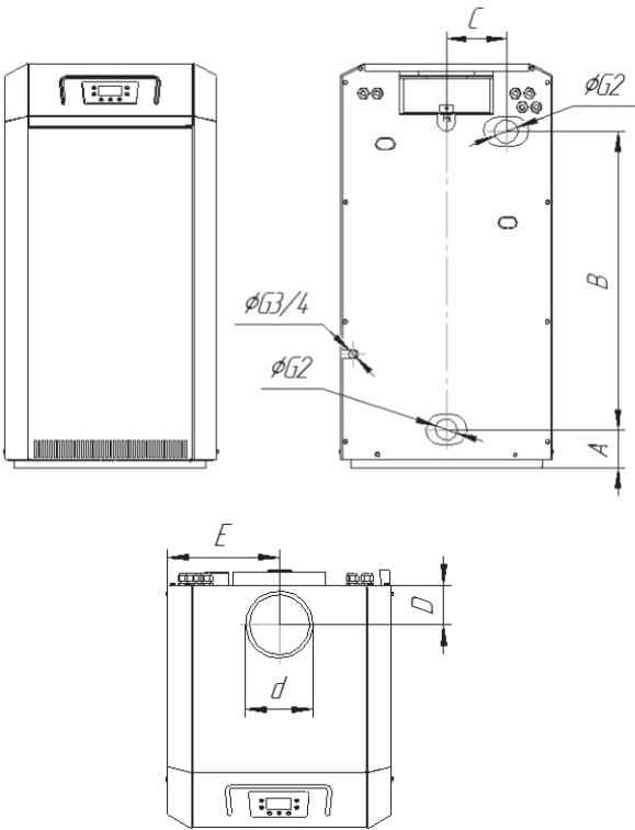
CLEVER-20/30/40
