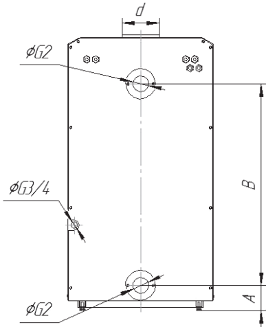
CLEVER-55
