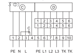
ZPE 800 L1 Compact (400 В,
