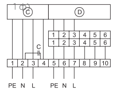
ZPE 800 L1 Compact (400 В,
