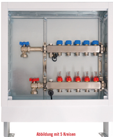
VA-FBif - TT-AGEs 1" - 110T
