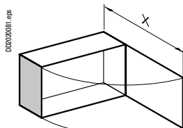
X = 577.5 (KSB160S●●) X = 777 (KSB250SE●) X = 855 (KSB400SE●)
