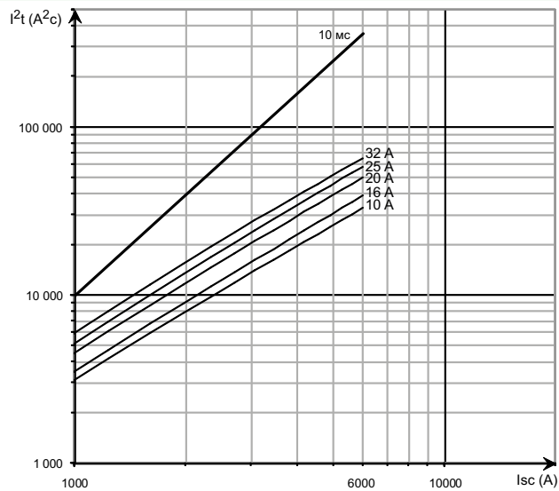
iC60 RCBO 6000 A - 3P/4P - 400 B
