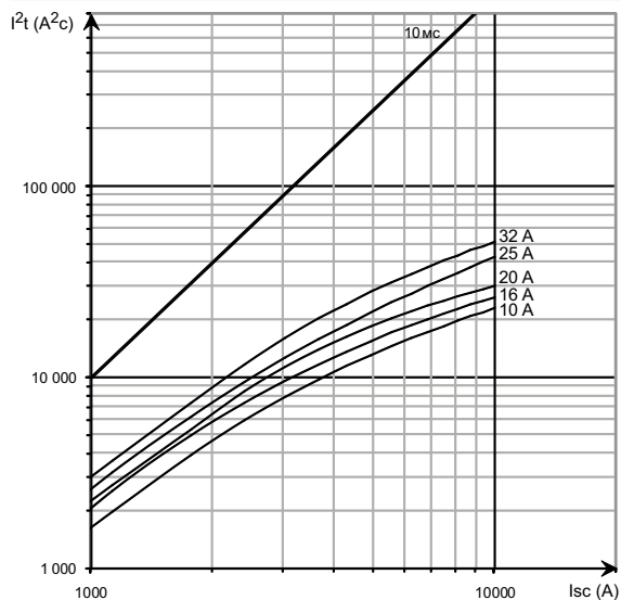
iC60 RCBO 10000 A - 2P/3P - 230 B
