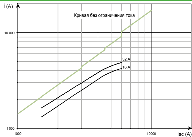
iC60 RCBO 6000 A - 3P/4P - 400 B
