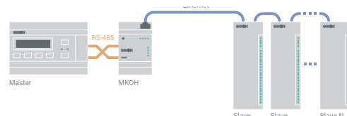
Master в cemu RS-485 – Slave в cemu Ethernet
