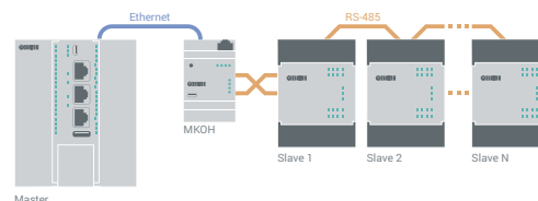
Master в cemu Ethernet – Slave в cemu RS-485
