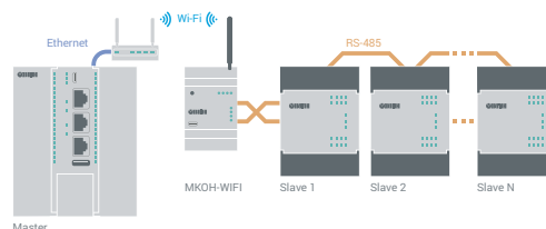
Master в cemu Wi-Fi – Slave в cemu RS-485
