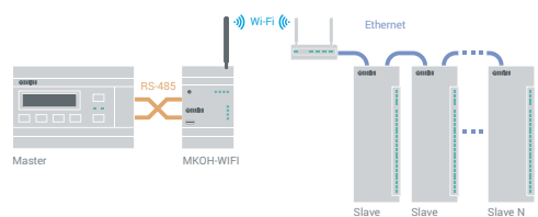
Master в cemu Wi-Fi – Slave в cemu RS-485
