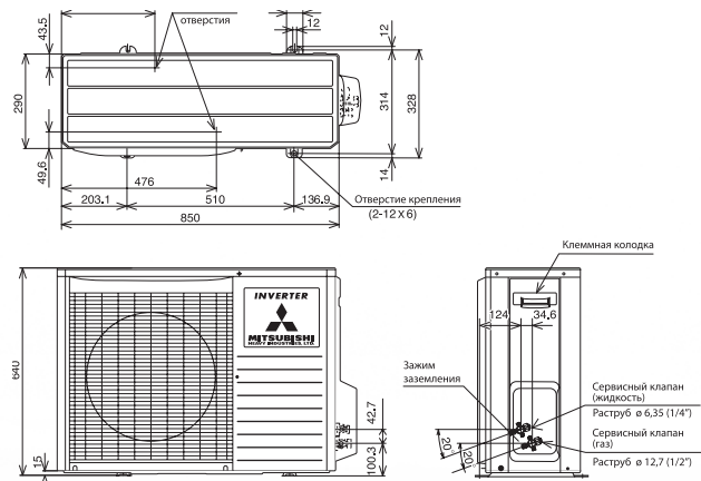
SRC50/56/63HE-S1
