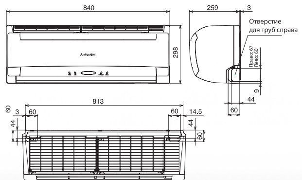
SRK50/56HE-S1
