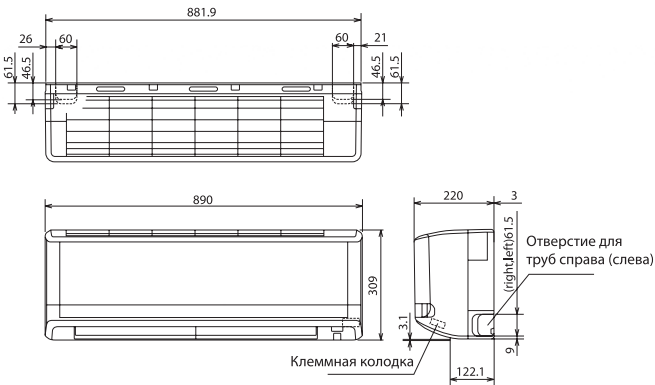
SRK20/25/35/50/60ZJX-S
