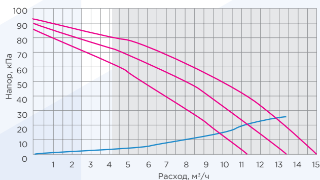
DV-UH 65-120-63.0-65
