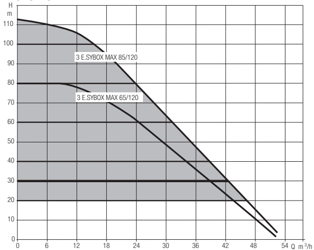
3 ESYBOX MAX
