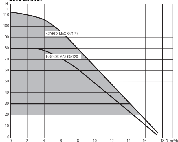
ESYBOX MAX
