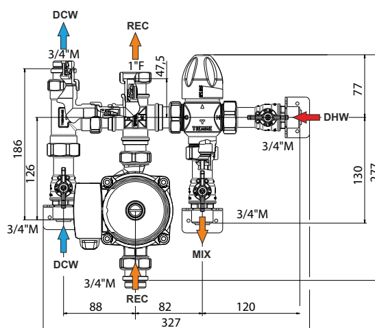
4738KR Anti-scald thermostatic kit with recirculation
