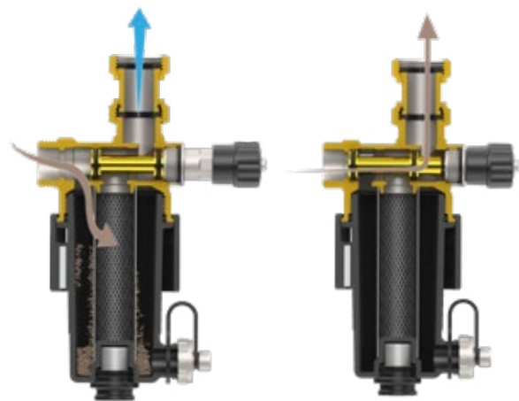
By-pass open: filter on
