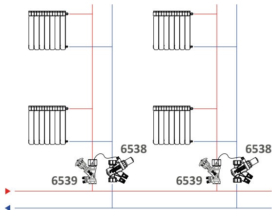
Diagram 1: Riser balancing function
