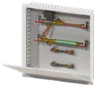
6500C0132V3 Pre-installation metal housing for "VARIO DN32" system, with 3-way zone valve. Setup stubs included.
