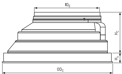
DN 1000
