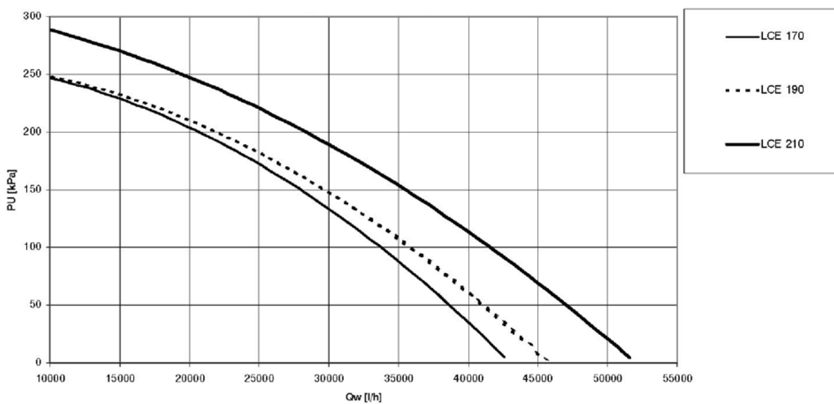
Standard pump available heat, LCE frame 1 - 2 - 3 - single or double "OR" operation -
