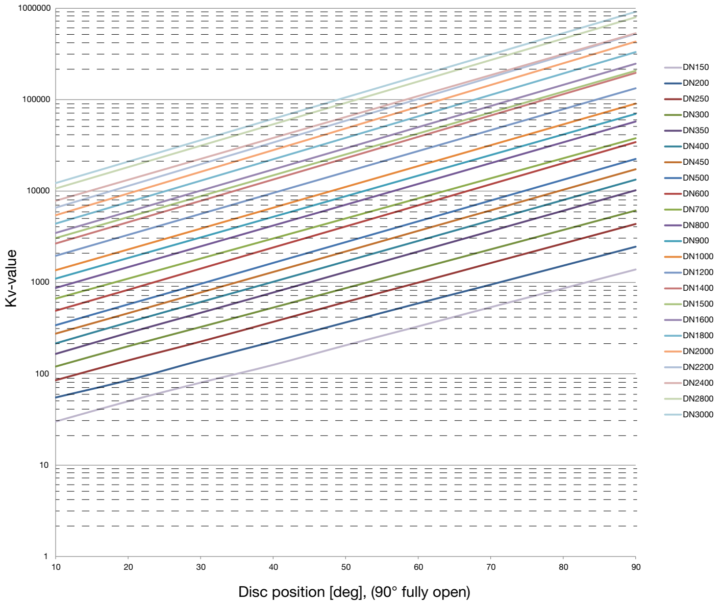
Kv values, butterfly valves DN150 - 3000, S756 - Plate disc
