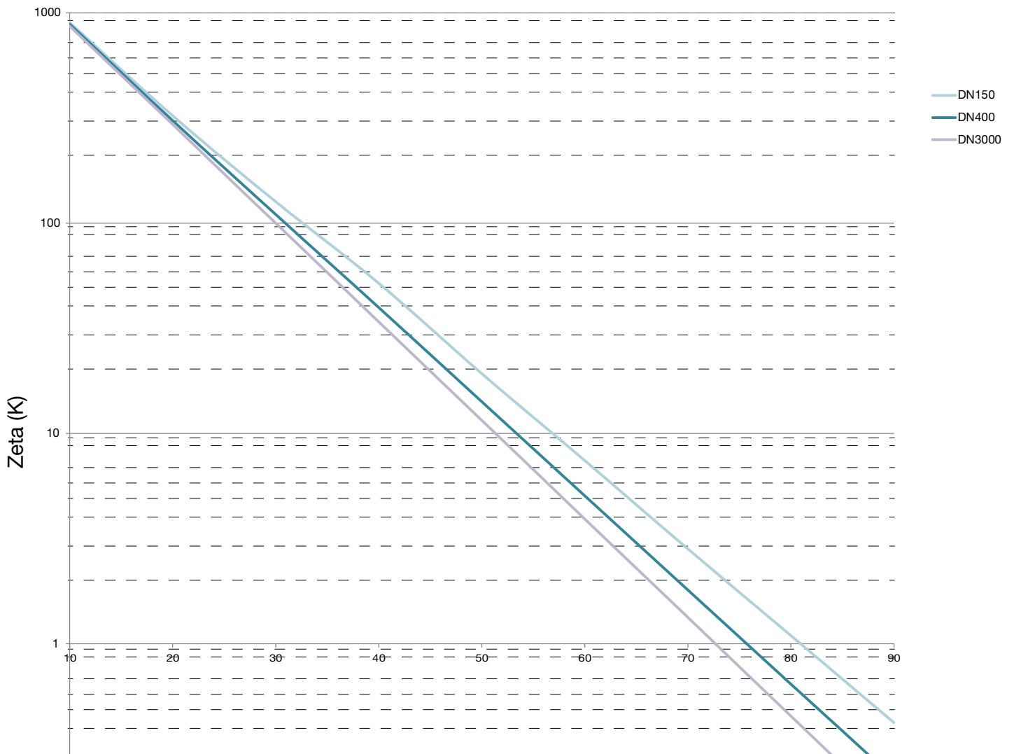
Zeta (K) value, butterfly valves DN150 - 3000, S756 - Plate disc
