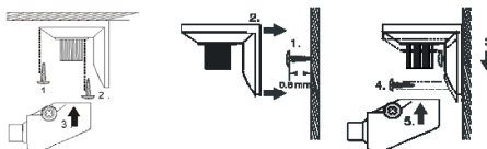
Fig.2 Installation of the mounting bracket
