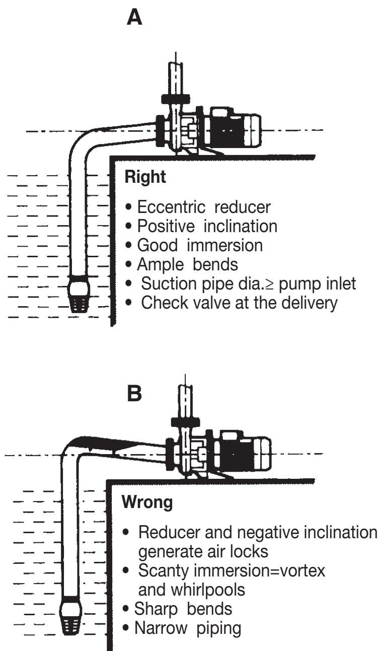
fig. 1 - Pump installation
