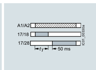
3RP257..NW30, 2 NO, wye-delta function
