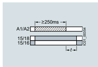
3RP2540..A.30, 1 CO, OFF-delay (N) 1)
