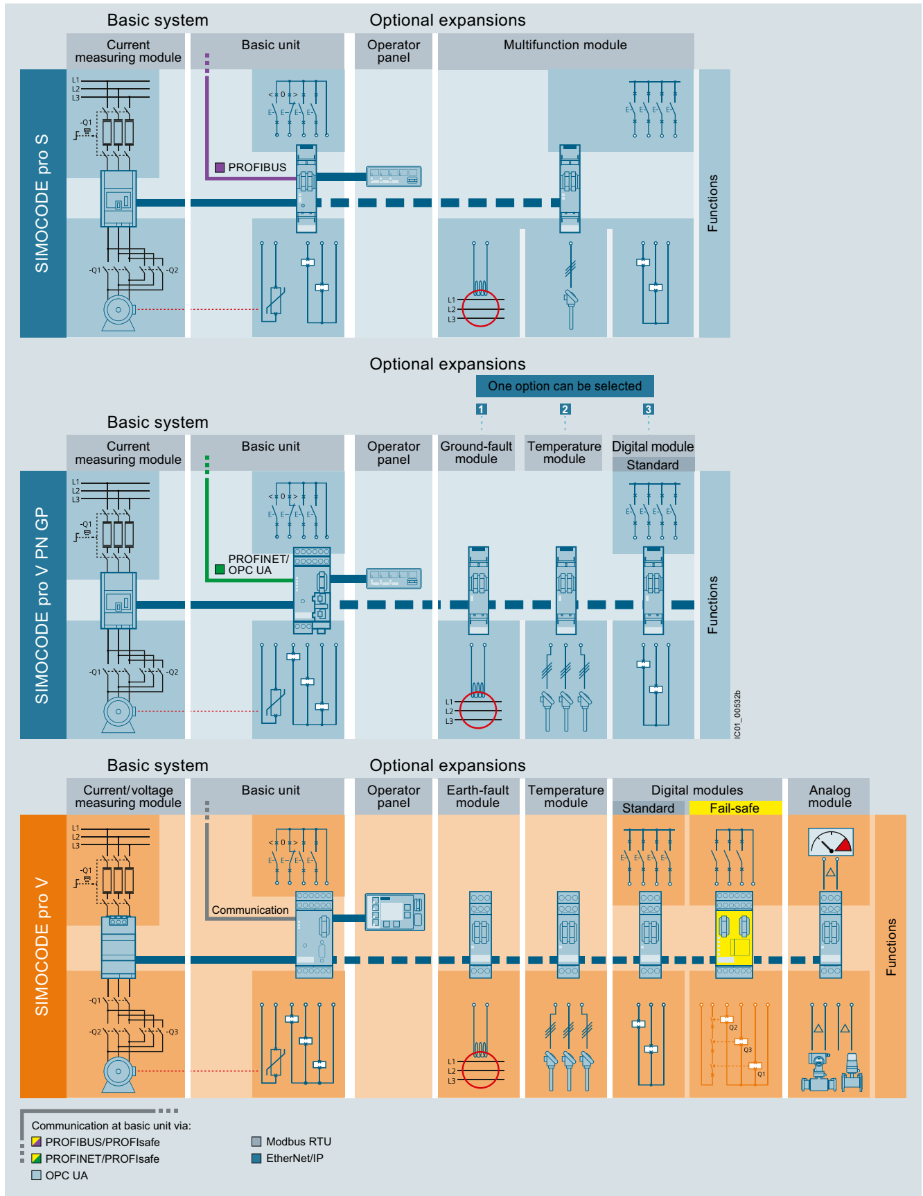
System structure
