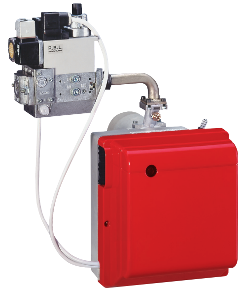
Gas train installed on the burner
