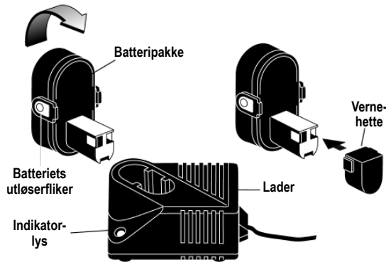
Figur 4 – Lade batteripakken
