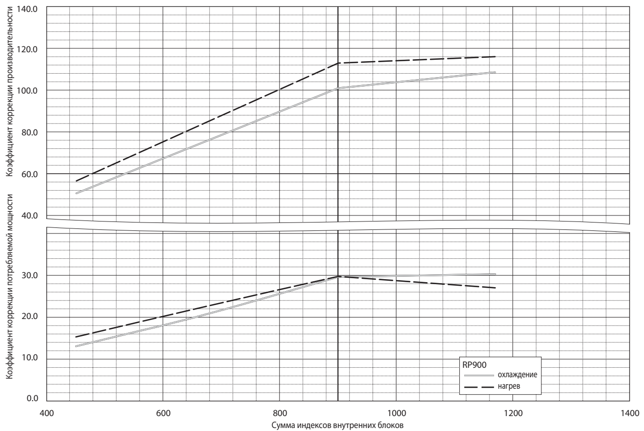
PUHY-RP900YSJM-B (-BS)
