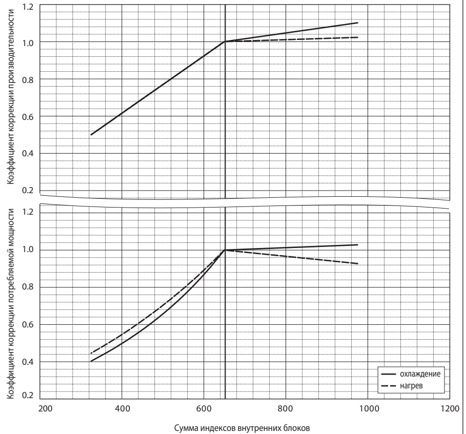
PURY-EP650YSJM-A
