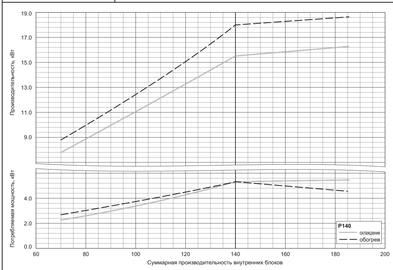
PUMY-P140YHMB
