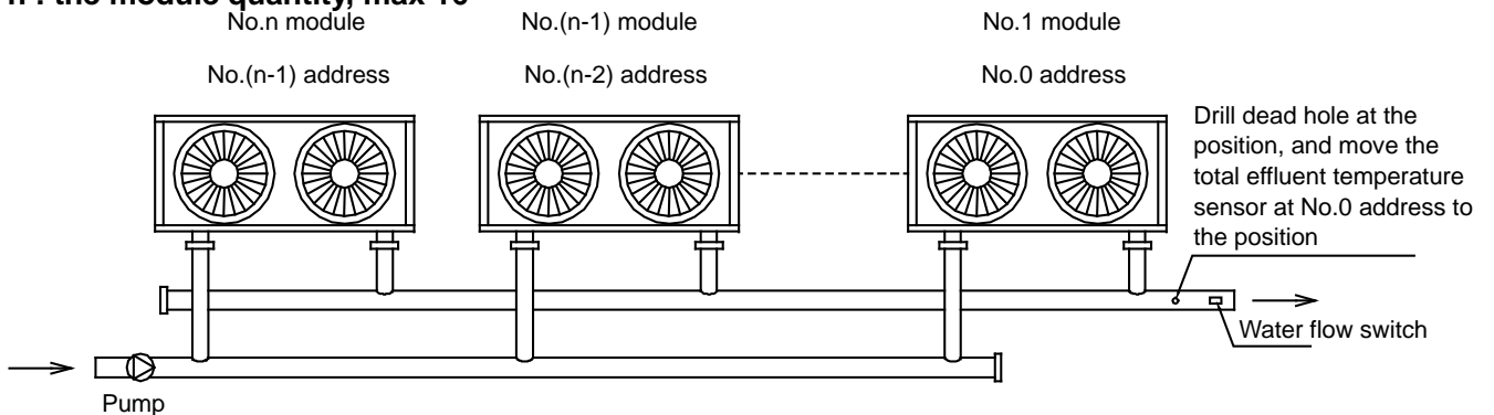
Installation mode A: less than 16 modules
