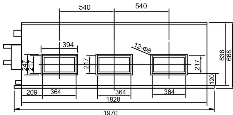
View of air inlet side (Unit: mm)
