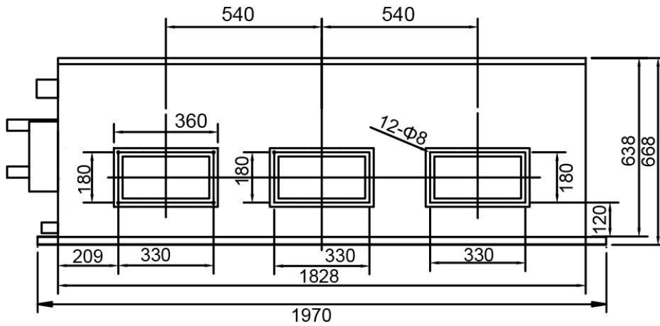
View of air outlet side (Unit: mm)
