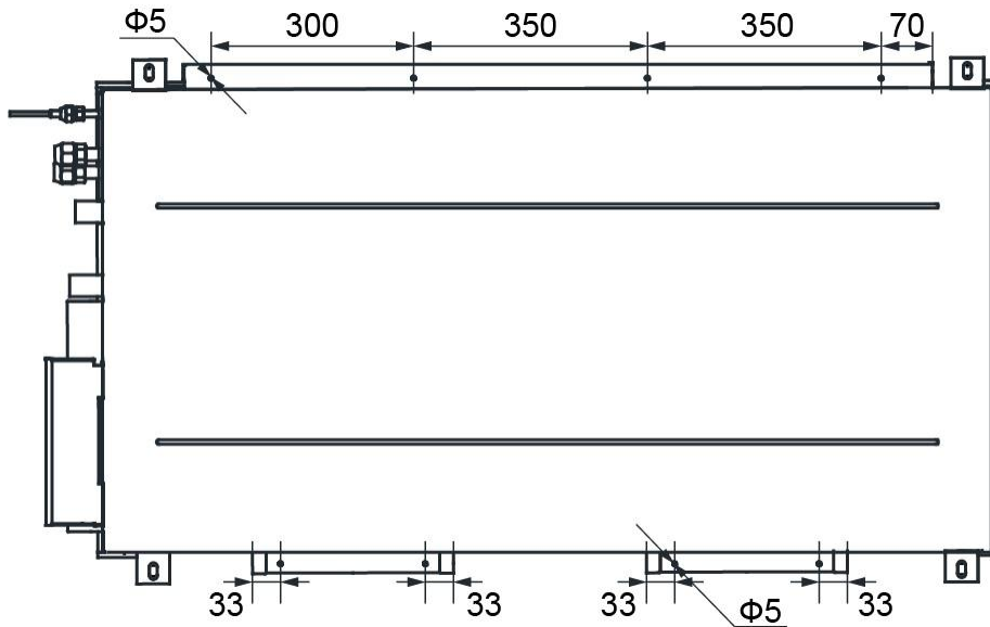
View of top side (Unit: mm)
