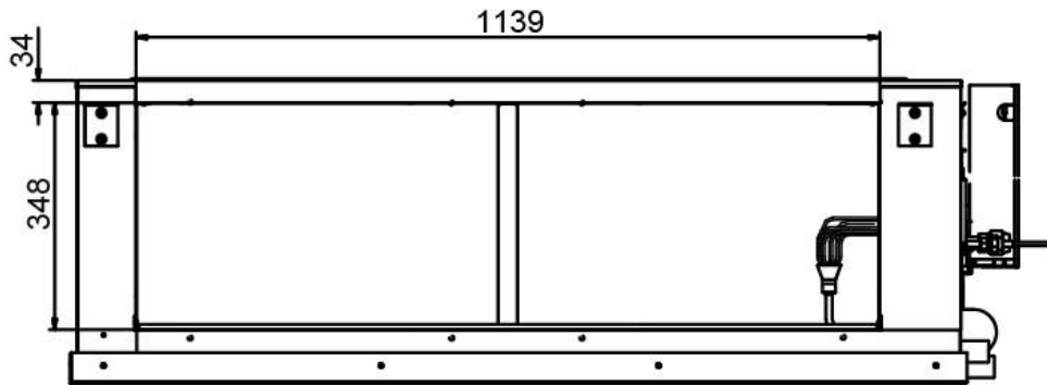
View of air inlet side
