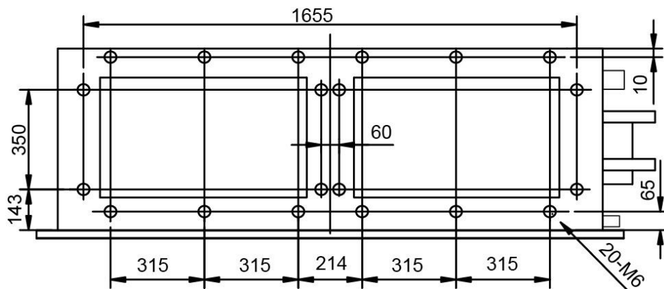
View of air inlet side (Unit: mm)
