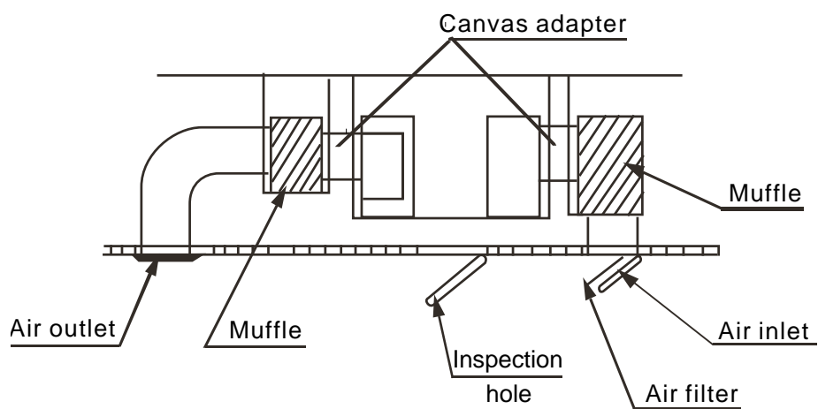
Air duct system
