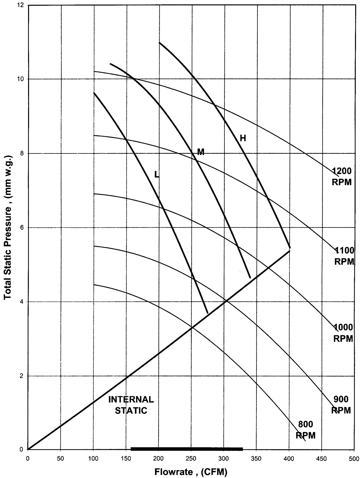
BLOWER PERFORMANCE CURVE MCC 010CW
