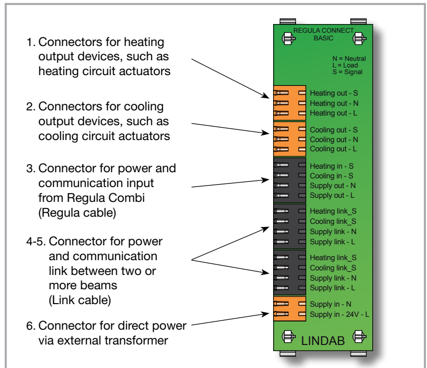
Figure 6. Connection card.
