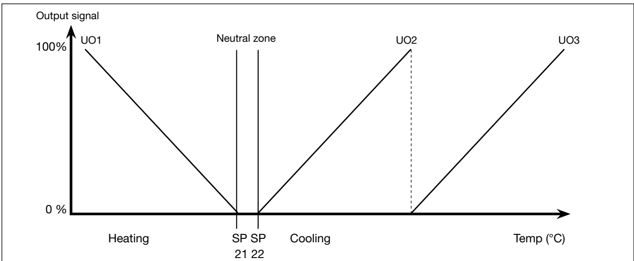
Diagram 1. Temperature sequences for program 1 water.
