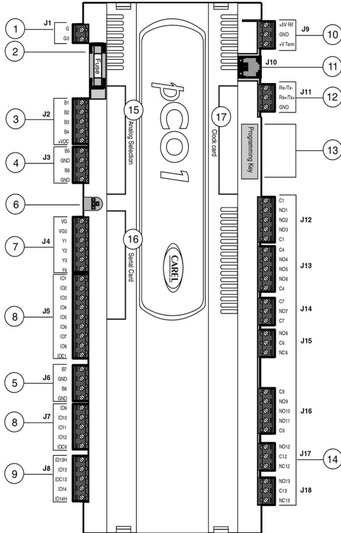
Figure 15: Layout
