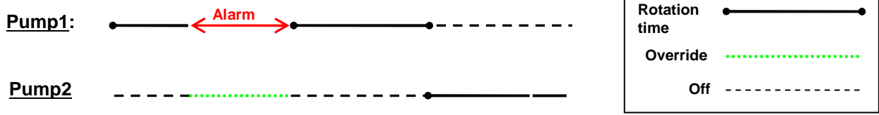
Figure 14: Pump Rotation with Alarm - 1
