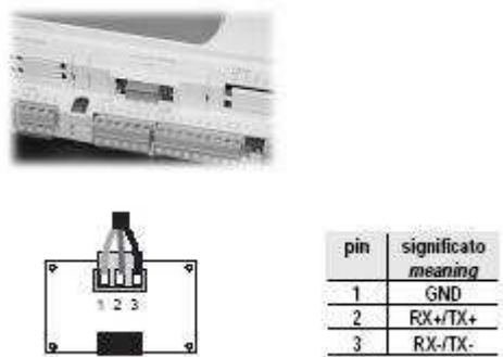
Figure 30: RS485 Serial Card
