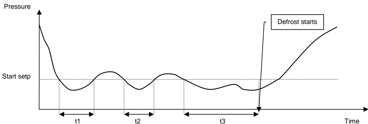
Figure 18: Threshold Logic
