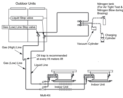
Example of Evacuation and Refrigerant Charge for FSN
