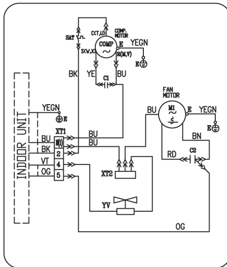
Модели GWHN09AANK3A1A/O, GWHN12ABNK3A1A/O – наружный блок
