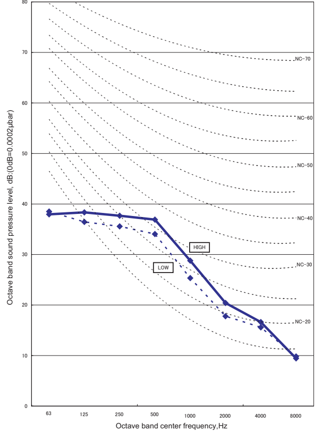
● MODEL : AR*14U
