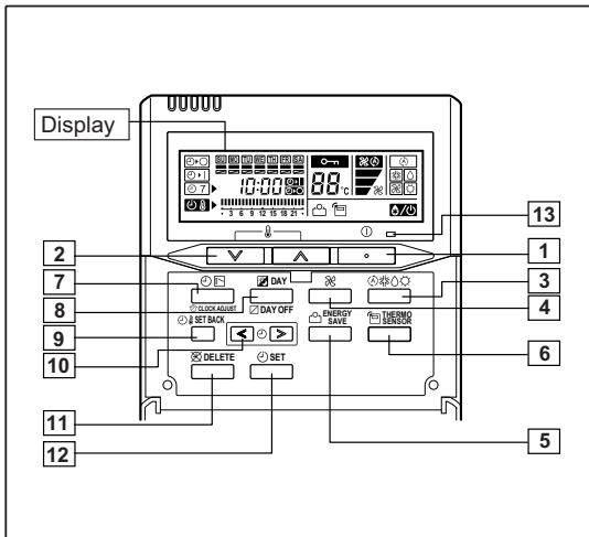
Display panel
