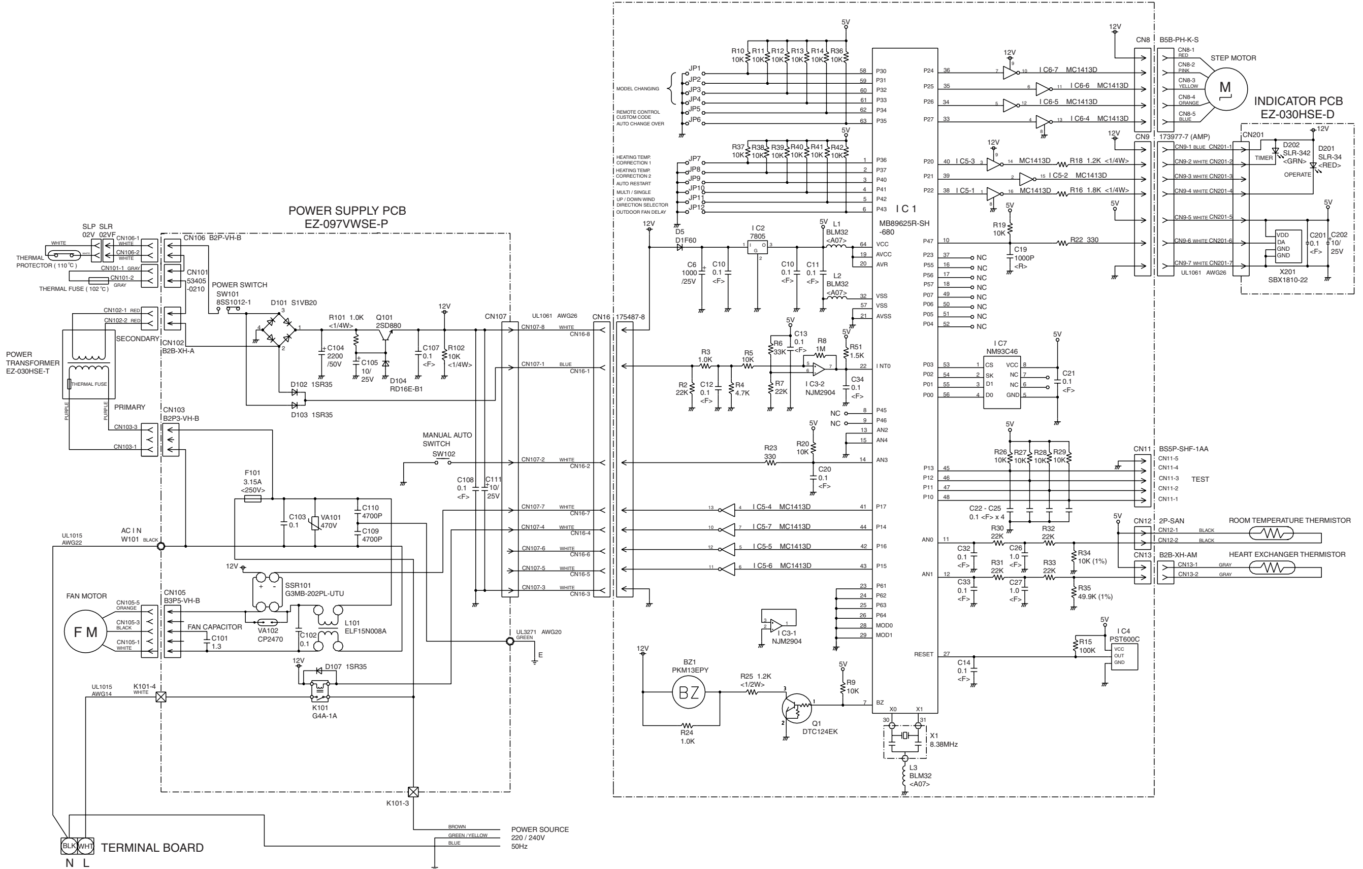
CONTROLLER PCB ASSEMBLY ( MAIN PCB ) EZ-095GWSE-C ( F )
