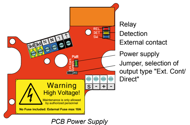
PCB Power Supply
