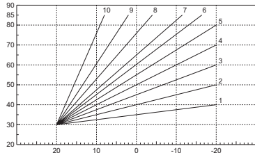
fig. 14 - Compensation curves
