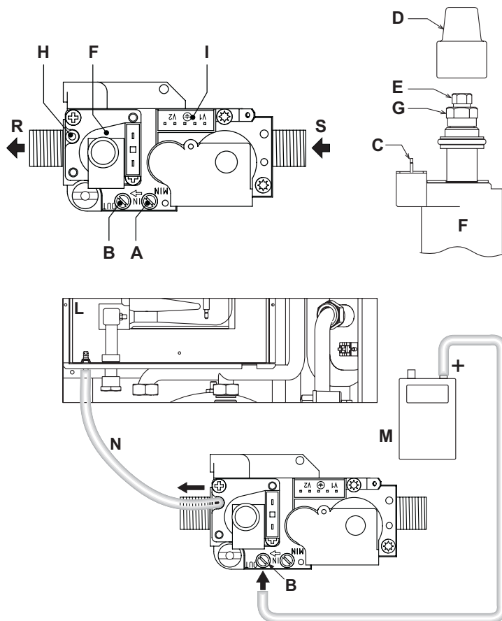
fig. 27 - Gas valve
