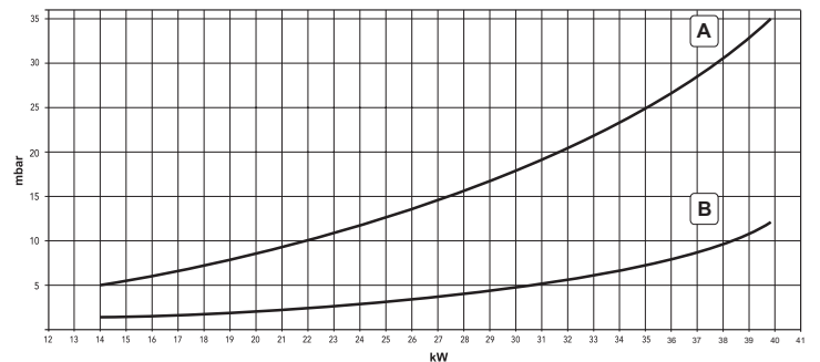
fig. 37 - Pressure - power diagram DIVAtop MICRO F 37
