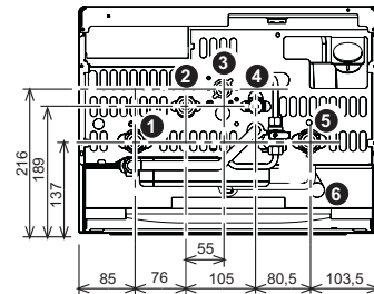
fig. 17 - Raccordements hydrauliques
